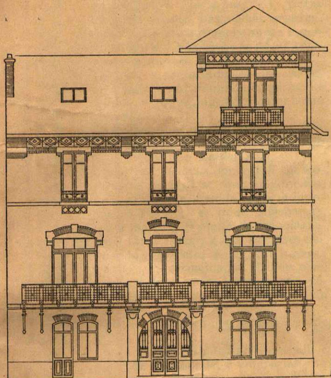
FACHADA PRINCIPAL
